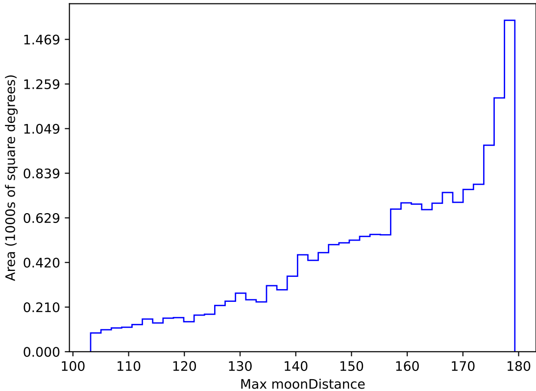
ddf_acor_sf30_lsf40_lsr10_v3.4_10yrs WFD r band: Max moonDistance
