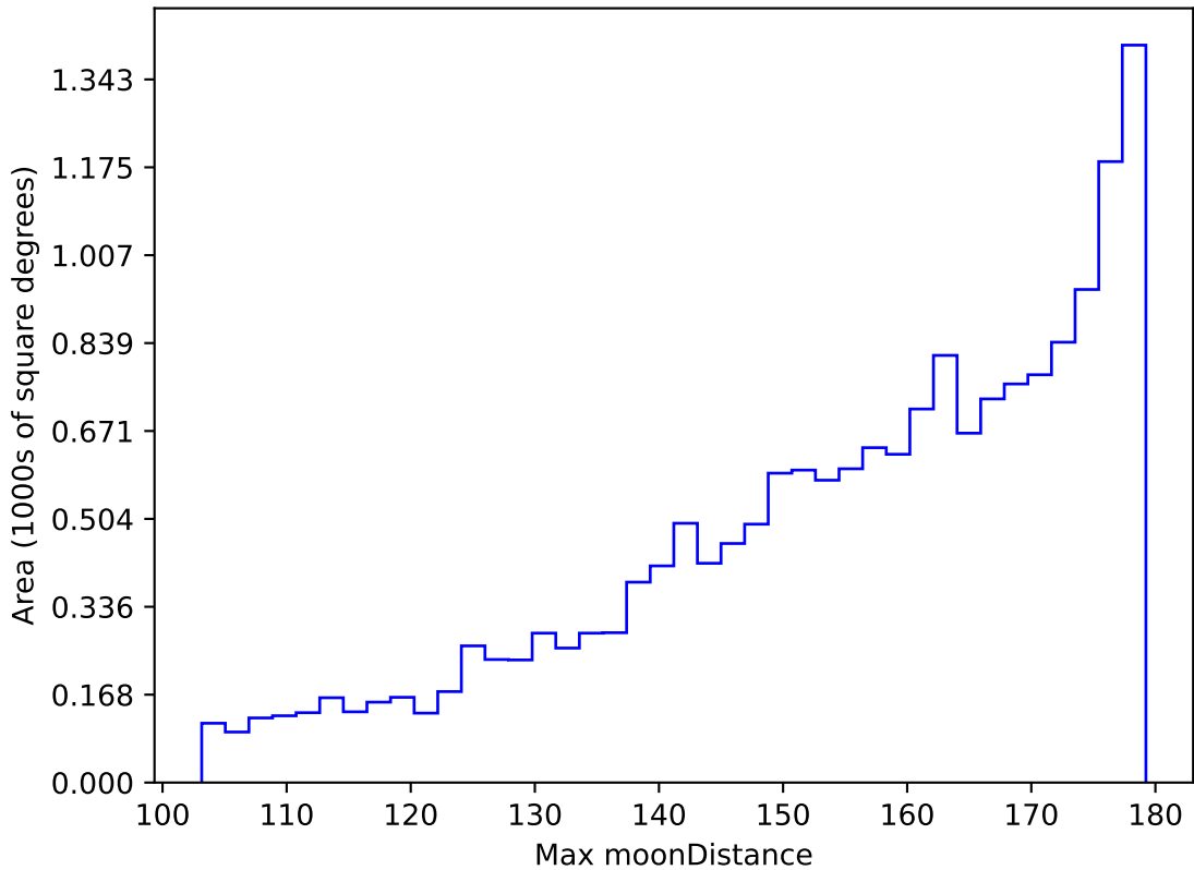
ddf_acor_sf30_lsf40_lsr10_v3.4_10yrs WFD i band: Max moonDistance
