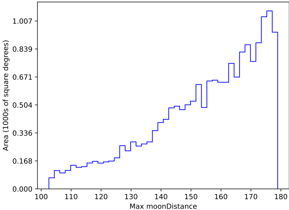
ddf_acor_sf30_lsf40_lsr10_v3.4_10yrs WFD g band: Max moonDistance
