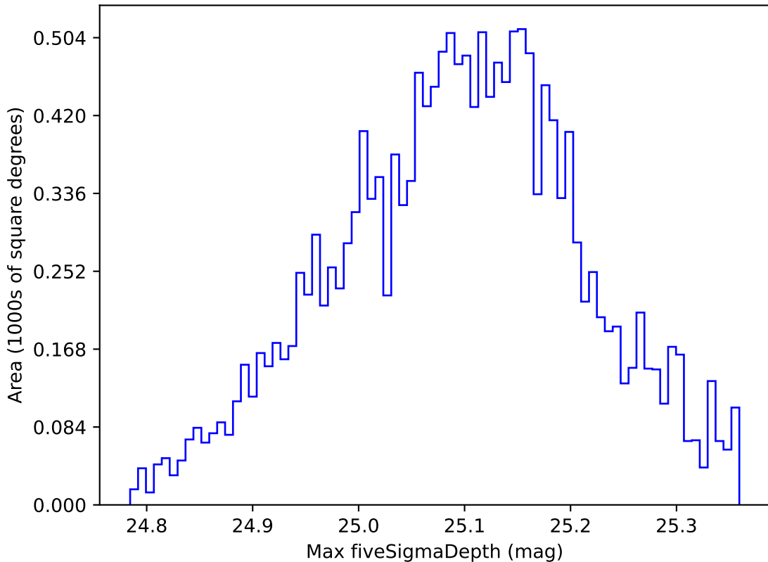
ddf_acor_sf30_lsf40_lsr10_v3.4_10yrs WFD all bands: Max fiveSigmaDepth
