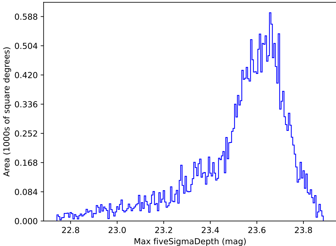
ddf_acor_sf30_lsf40_lsr10_v3.4_10yrs All sky z band: Max fiveSigmaDepth
