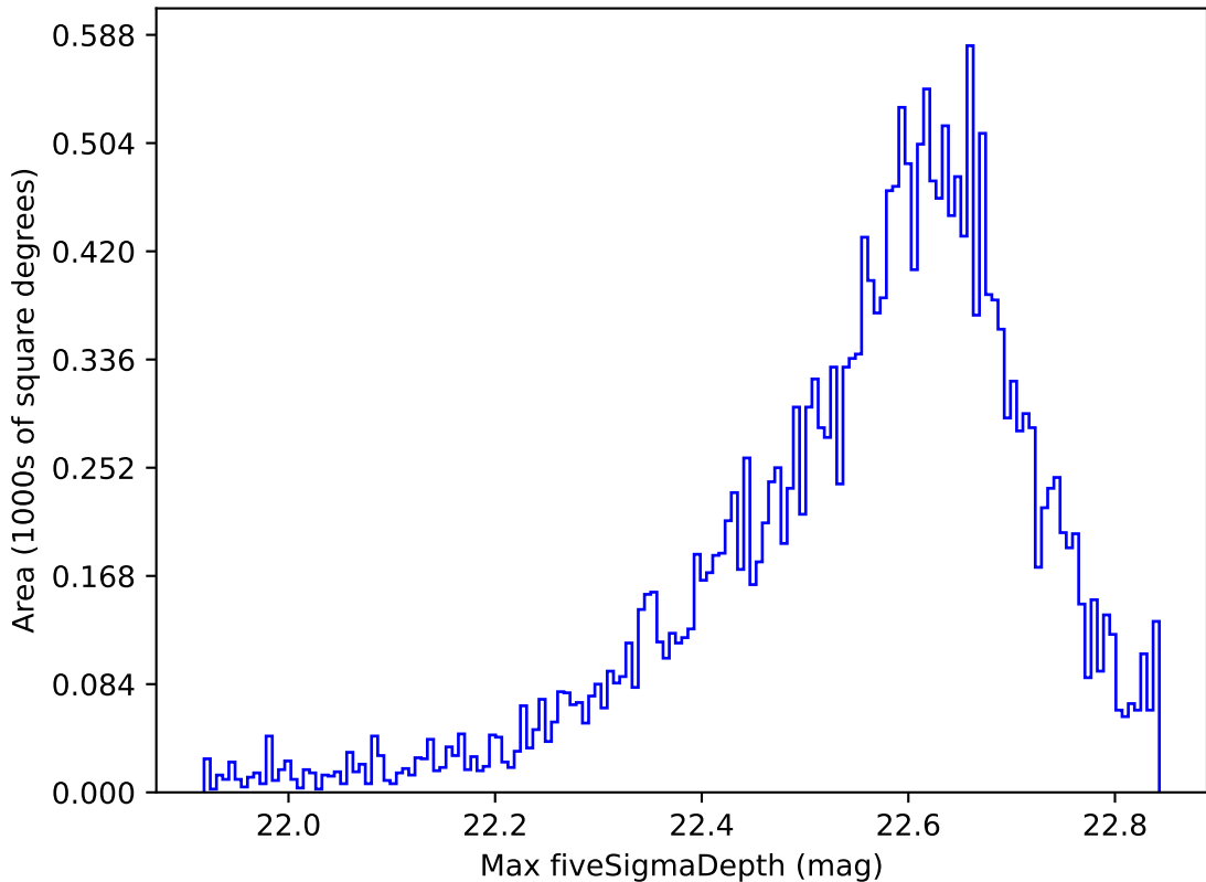
ddf_acor_sf30_ls40_lsr10_v3.4_10yrs All sky y band: Max fiveSigmaDepth
