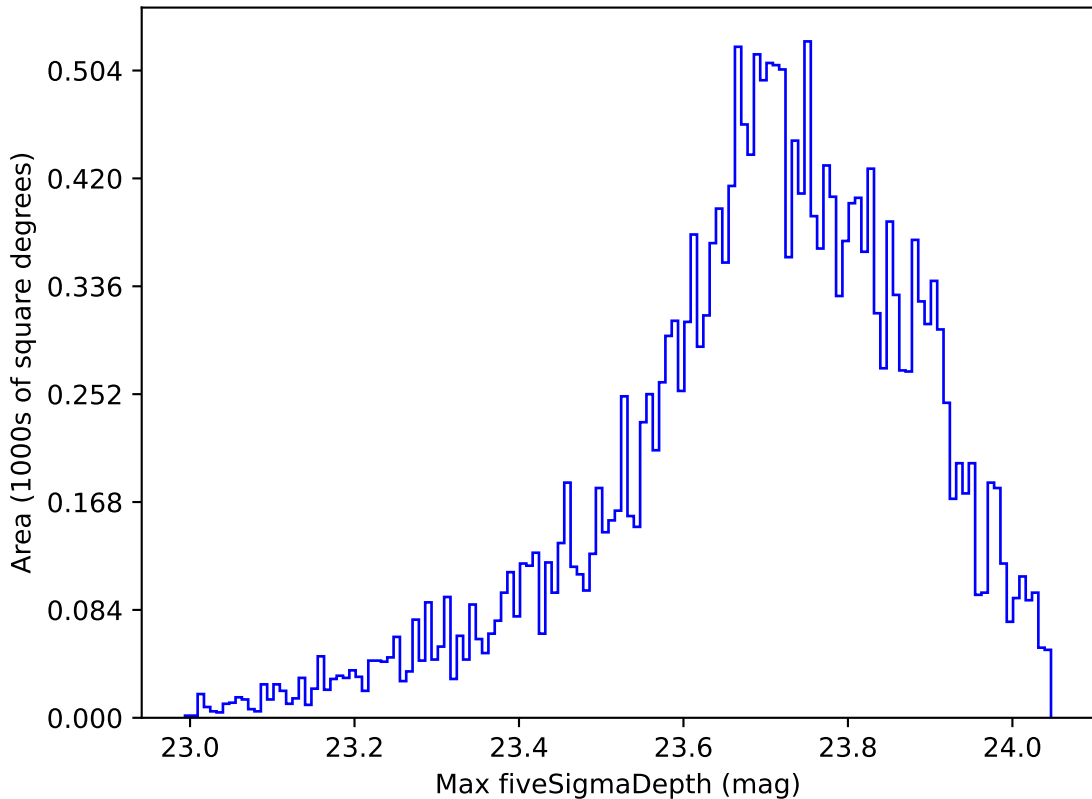
ddf_acor_sf30_lsf40_lsr10_v3.4_10yrs All sky u band: Max fiveSigmaDepth
