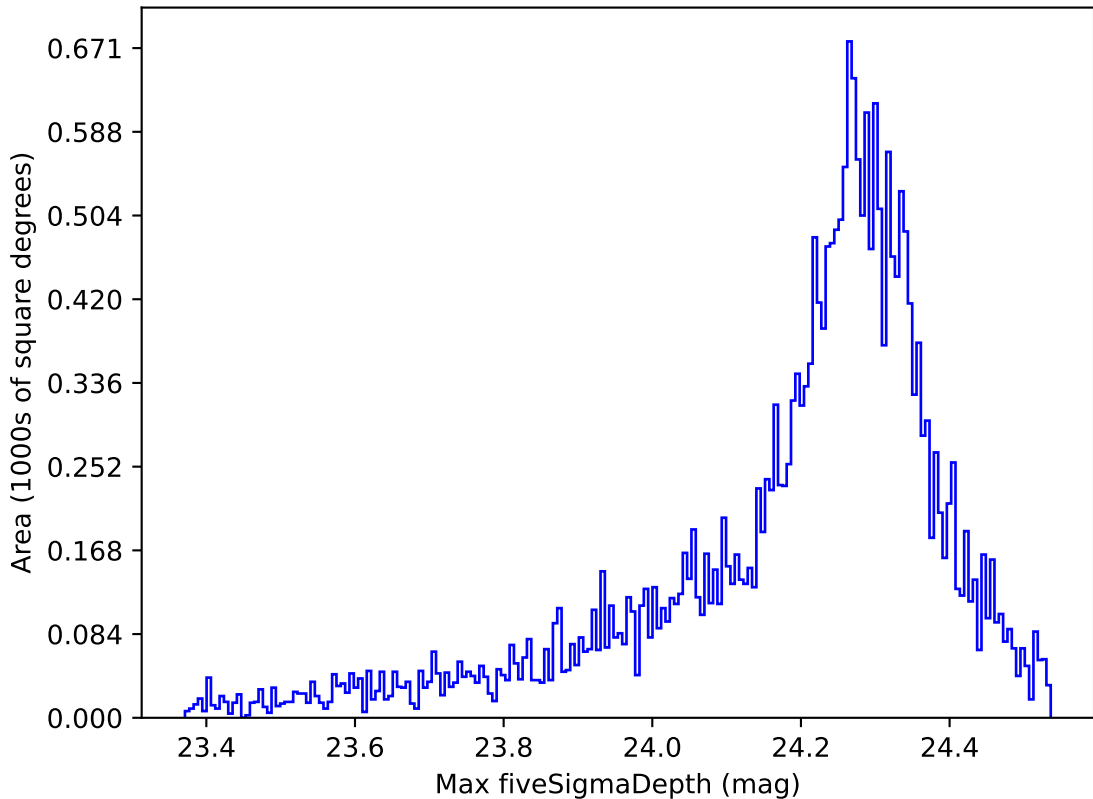
ddf_acor_sf30_lsf40_lsr10_v3.4_10yrs All sky i band: Max fiveSigmaDepth
