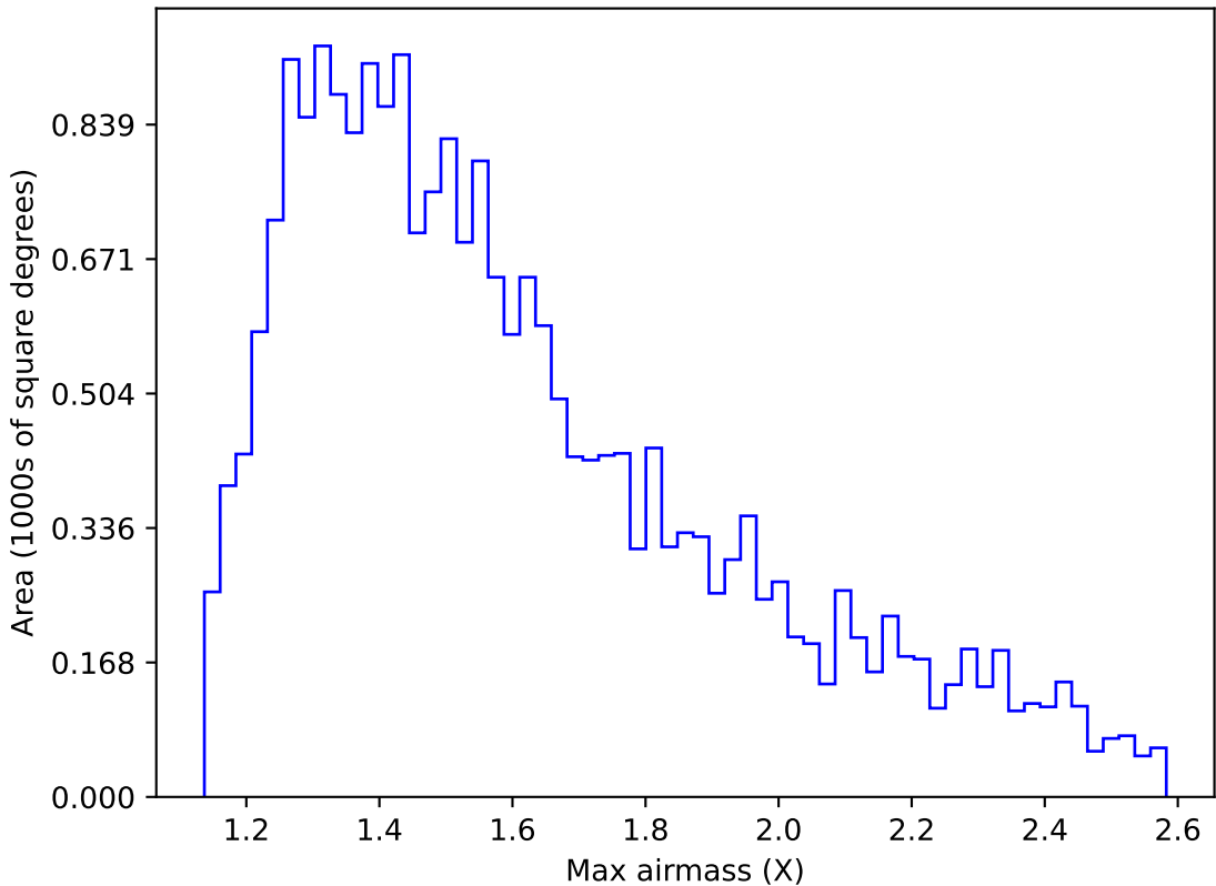
ddf_acor_sf30_lsf40_lsr10_v3.4_10yrs Yr 1 y band: Max airmass
