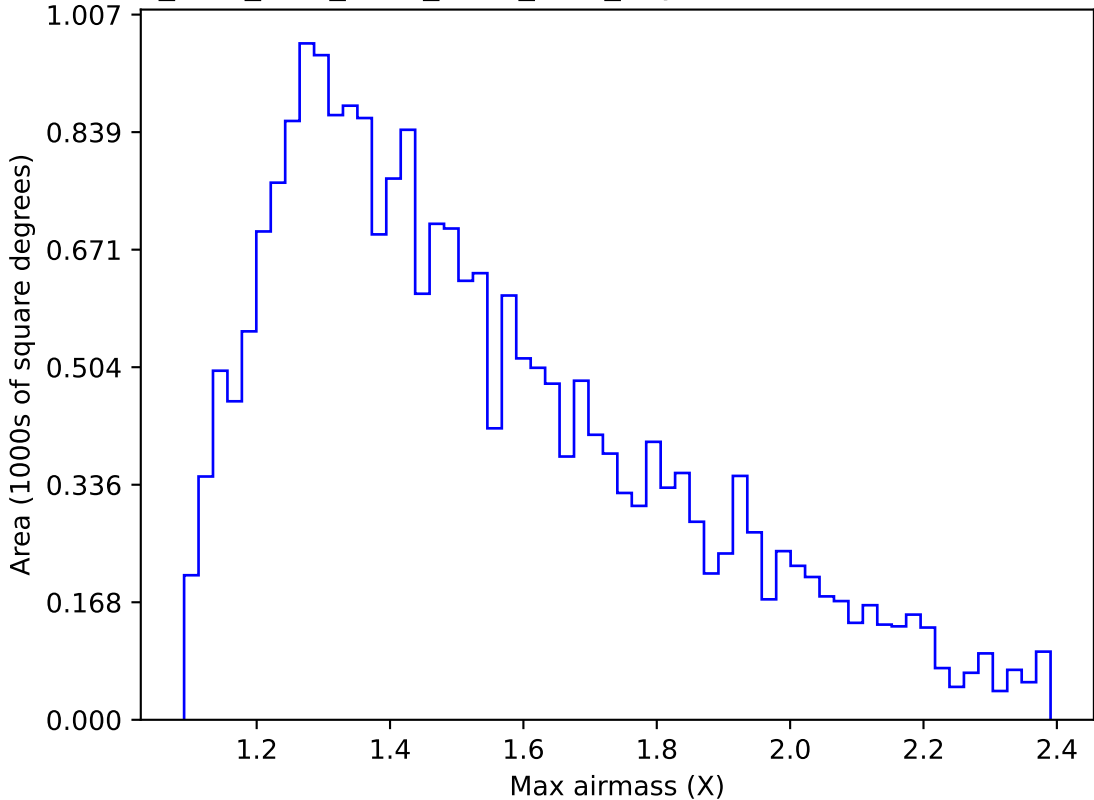
ddf_acor_sf30_lsf40_lsr10_v3.4_10yrs Yr 1 u band: Max airmass
