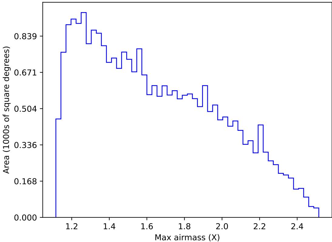
ddf_acor_sf30_lsf40_lsr10_v3.4_10yrs Yr 1 g band: Max airmass
