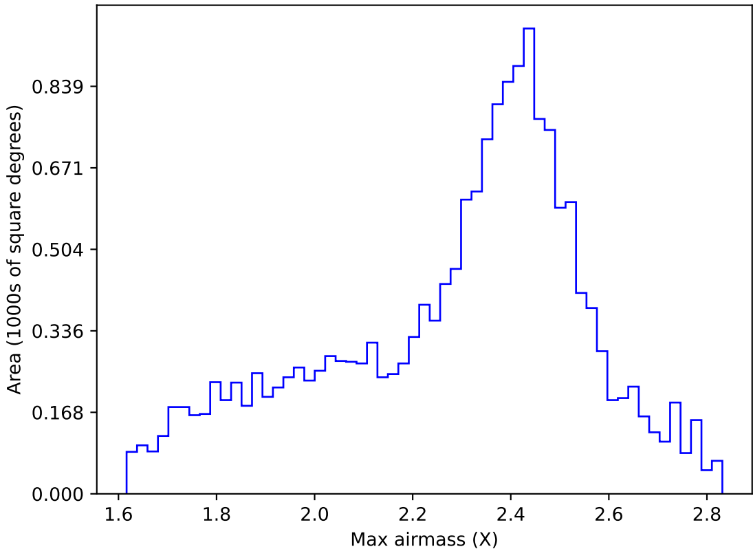
ddf_acor_sf30_lsf40_lsr10_v3.4_10yrs WFD r band: Max airmass
