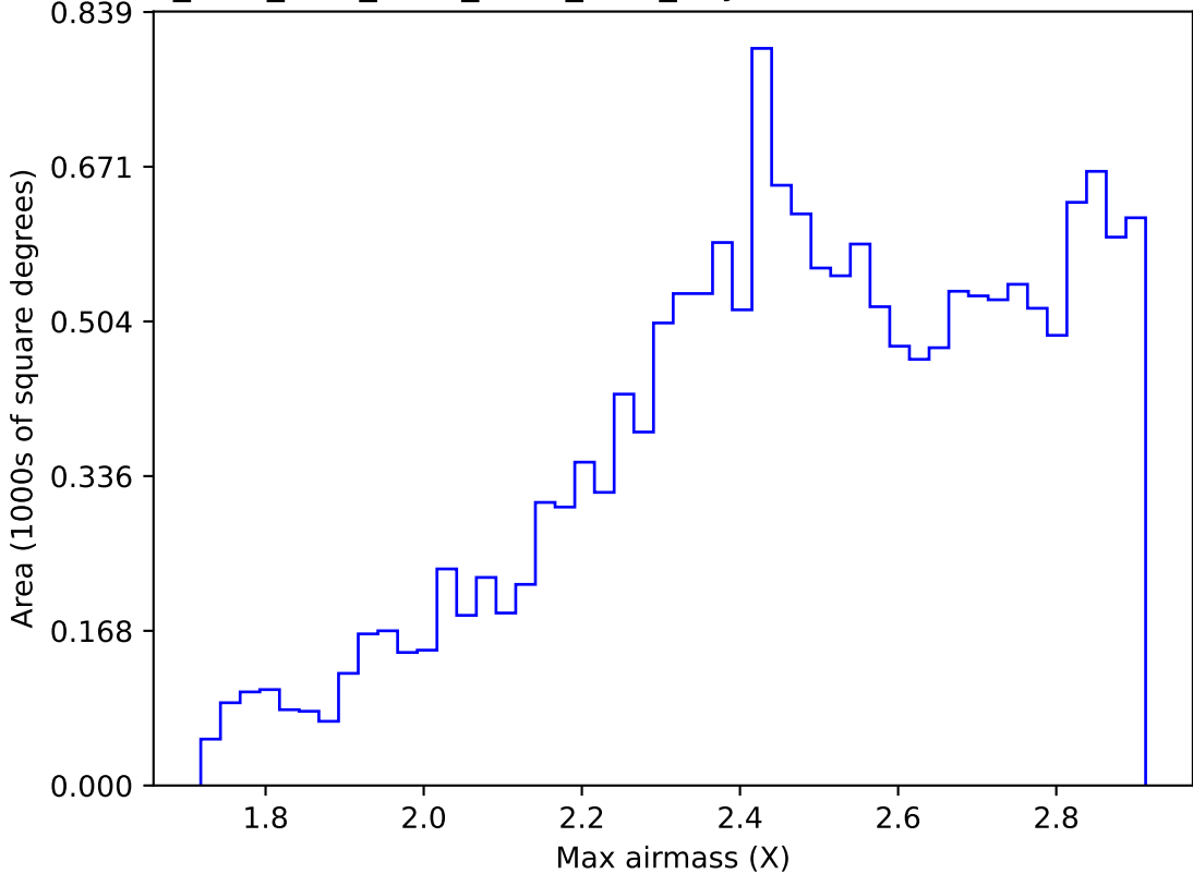
ddf_acor_sf30_lsf40_lsr10_v3.4_10yrs WFD i band: Max airmass
