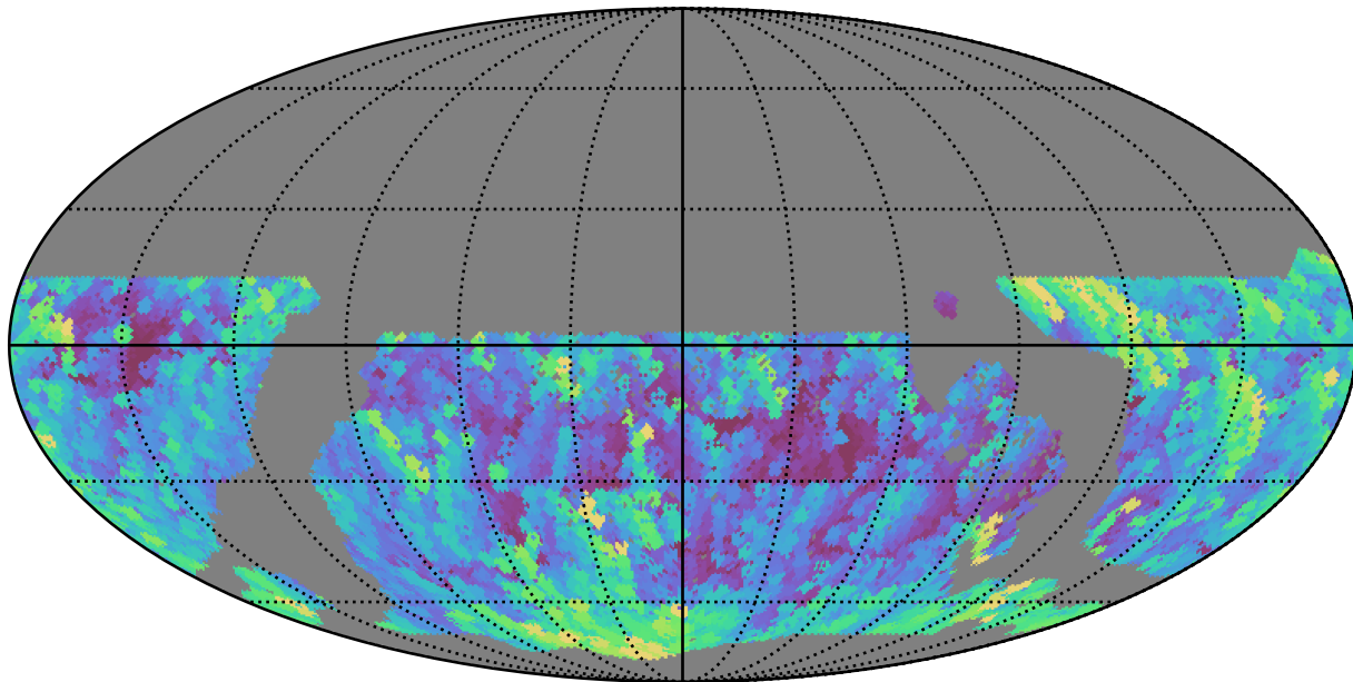
ddf_acor_sf30_lsf40_lsr10_v3.4_10yrs WFD g band: Max airmass
