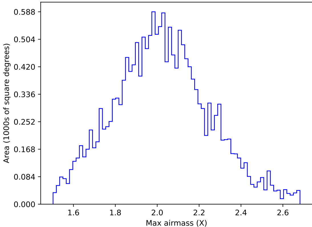
ddf_acor_sf30_lsf40_lsr10_v3.4_10yrs WFD g band: Max airmass
