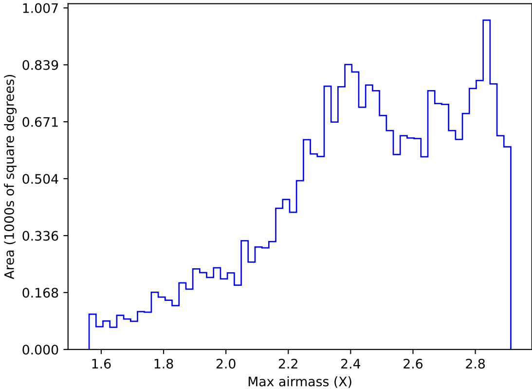
ddf_acor_sf30_lsf40_lsr10_v3.4_10yrs All sky z band: Max airmass
