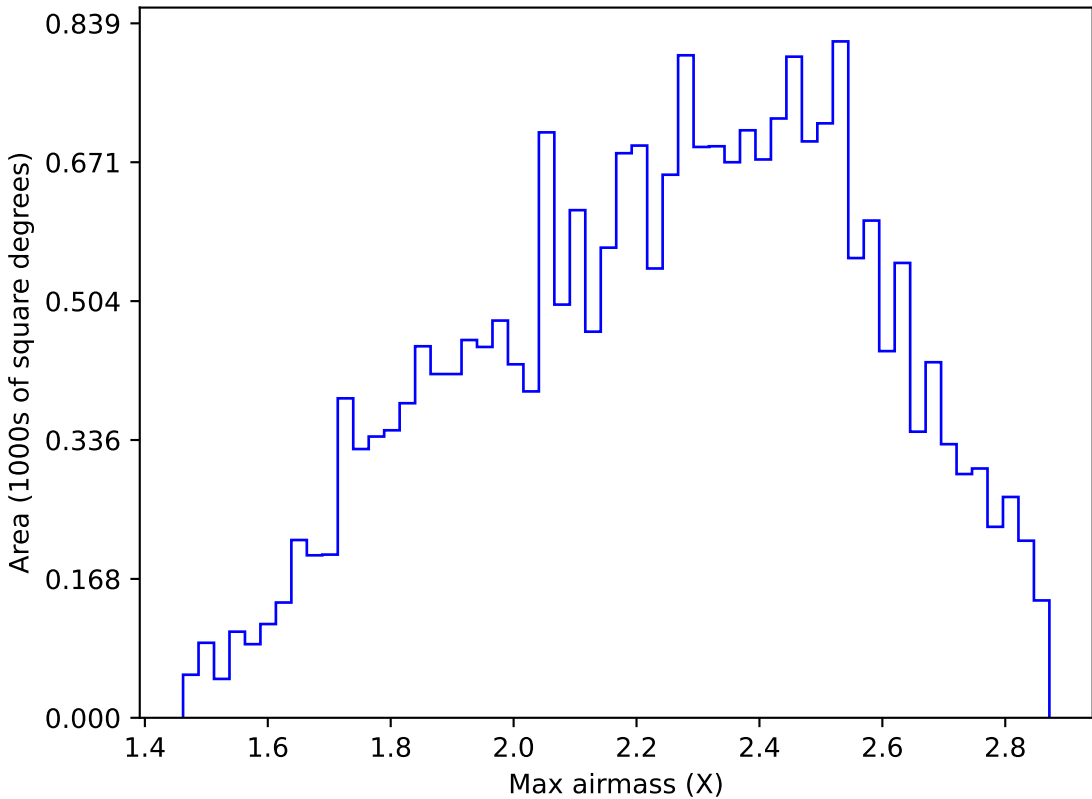
ddf_acor_sf30_lsf40_lsr10_v3.4_10yrs All sky y band: Max airmass
