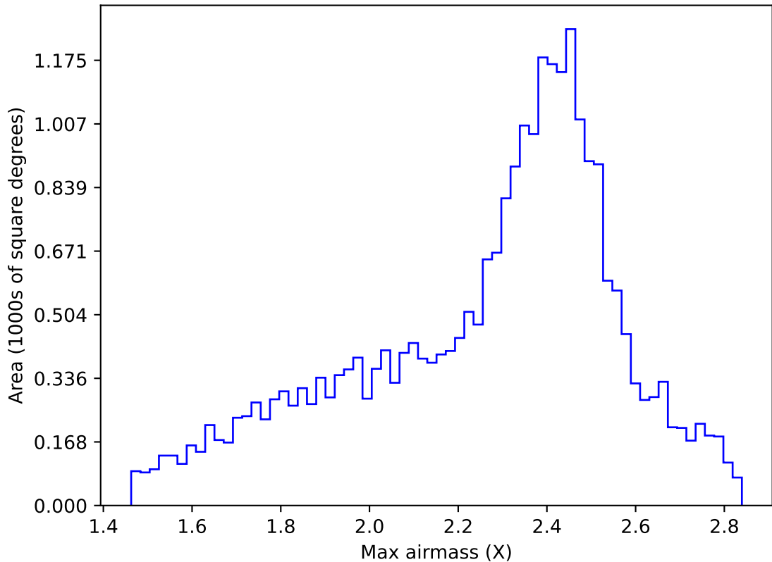
ddf_acor_sf30_lsf40_lsr10_v3.4_10yrs All sky r band: Max airmass
