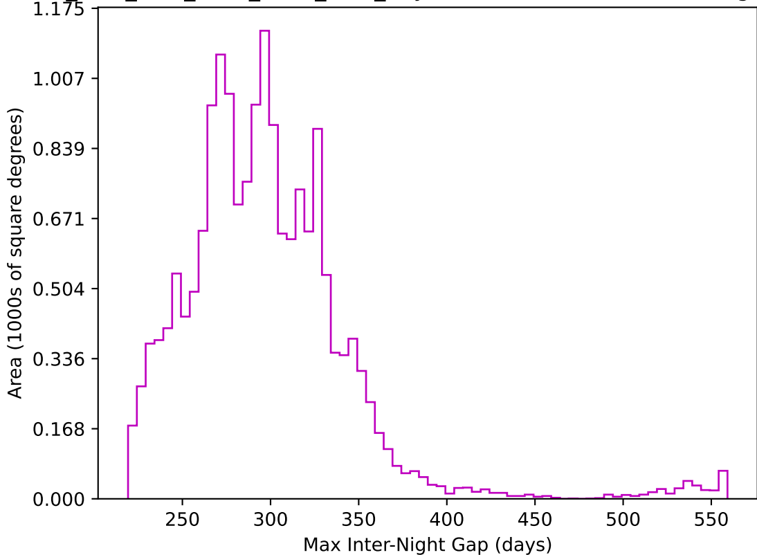
ddf_acor_sf30_lsf40_lsr10_v3.4_10yrs WFD z band: Max Inter-Night Gap
