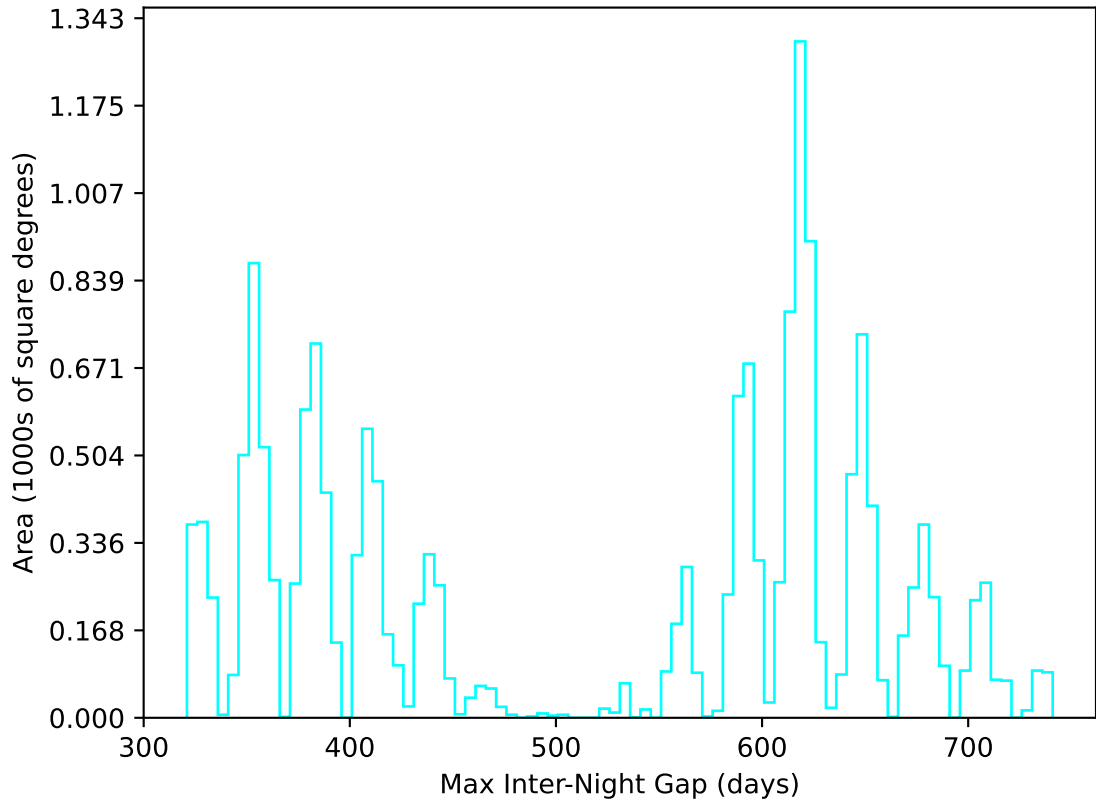
ddf_acor_sf30_lsf40_lsr10_v3.4_10yrs WFD u band: Max Inter-Night Gap
