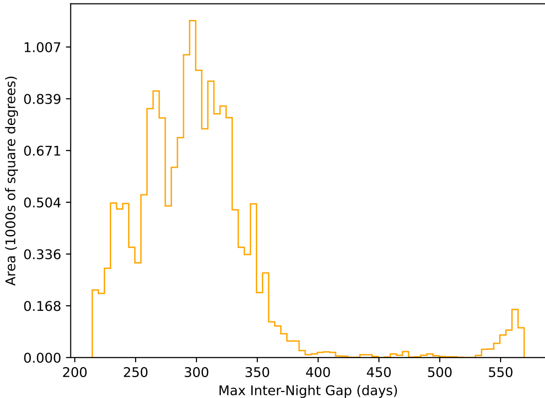
ddf_acor_sf30_lsf40_lsr10_v3.4_10yrs WFD r band: Max Inter-Night Gap
