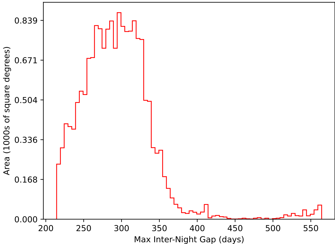
ddf_acor_sf30_lsf40_lsr10_v3.4_10yrs WFD i band: Max Inter-Night Gap
