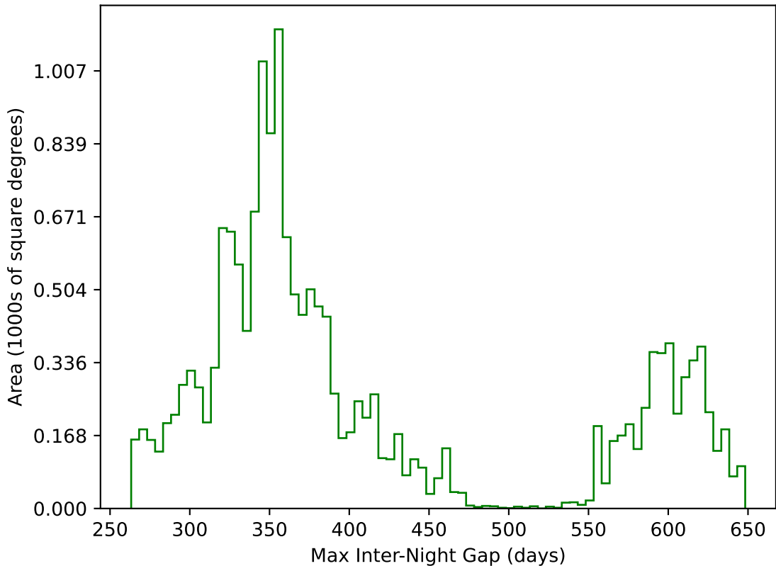
ddf_acor_sf30_lsf40_lsr10_v3.4_10yrs WFD g band: Max Inter-Night Gap
