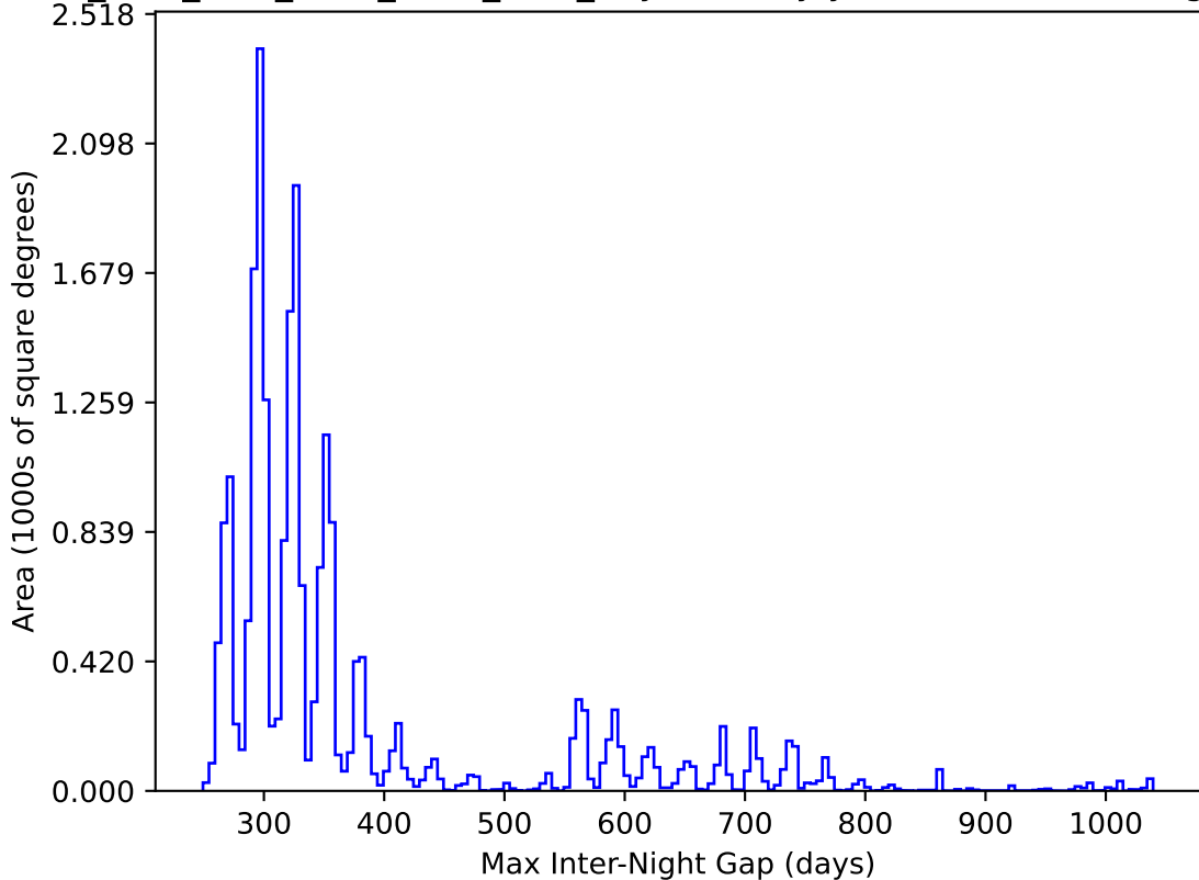
ddf_acor_sf30_lsf40_lsr10_v3.4_10yrs All sky y band: Max Inter-Night Gap
