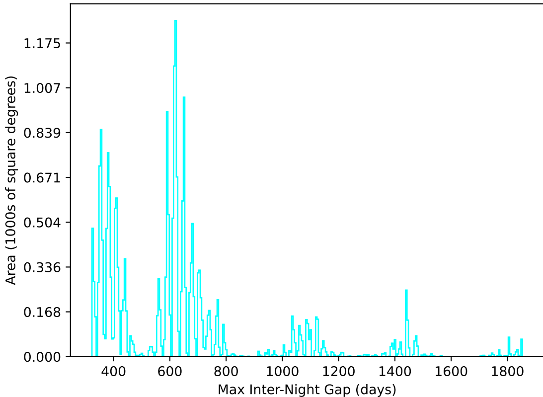
ddf_acor_sf30_lsf40_lsr10_v3.4_10yrs All sky u band: Max Inter-Night Gap
