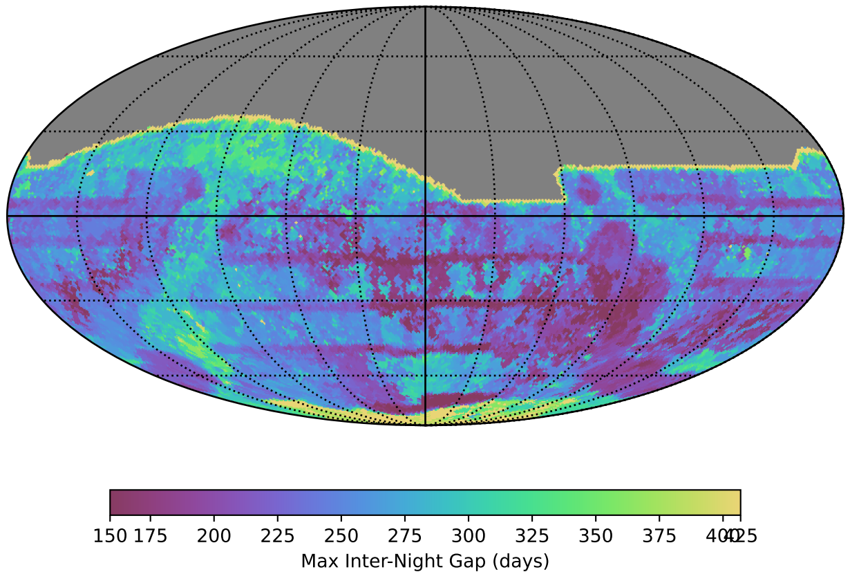
ddf_acor_sf30_lsf40_lsr10_v3.4_10yrs All sky all bands: Max Inter-Night Gap
