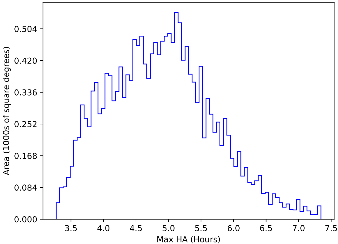
ddf_acor_sf30_lsf40_lsr10_v3.4_10yrs WFD z band: Max HA
