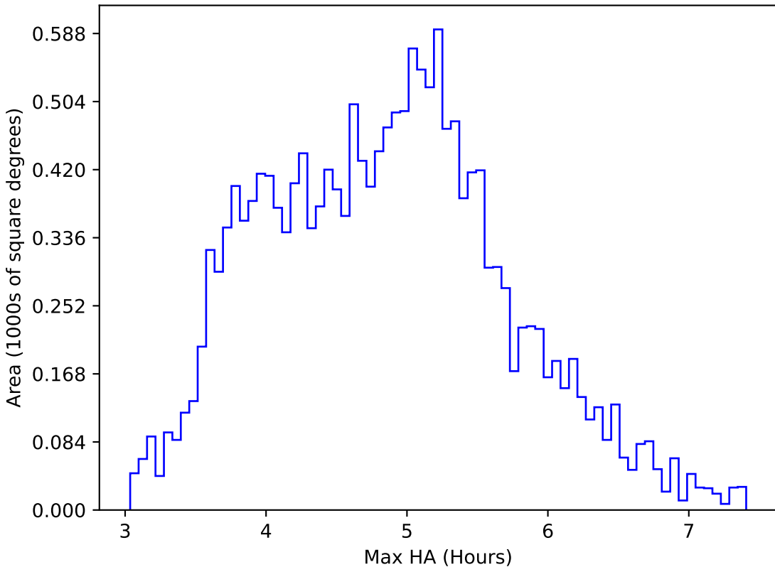
ddf_acor_sf30_lsf40_lsr10_v3.4_10yrs WFD i band: Max HA
