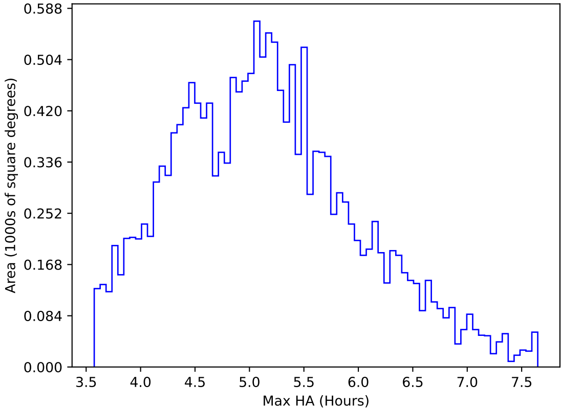
ddf_acor_sf30_lsf40_lsr10_v3.4_10yrs WFD all bands: Max HA
