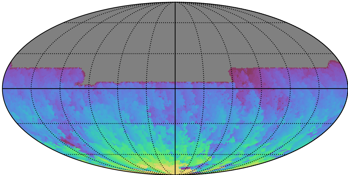
ddf_acor_sf30_lsf40_lsr10_v3.4_10yrs All sky y band: Max HA
