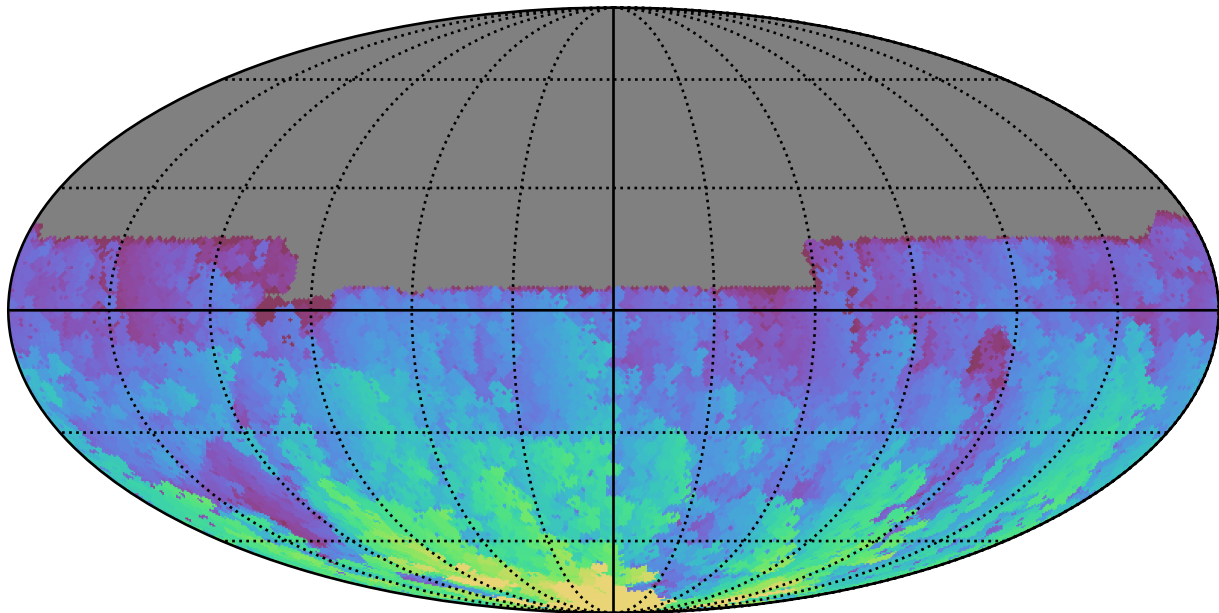
ddf_acor_sf30_lsf40_lsr10_v3.4_10yrs All sky u band: Max HA
