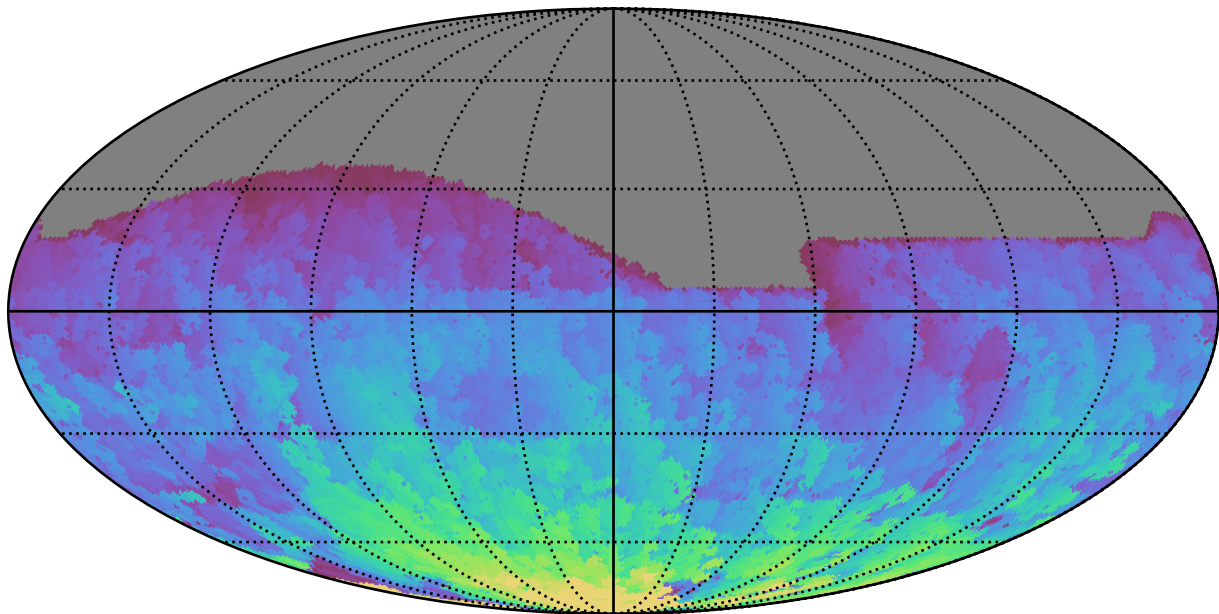
ddf_acor_sf30_lsf40_lsr10_v3.4_10yrs All sky r band: Max HA
