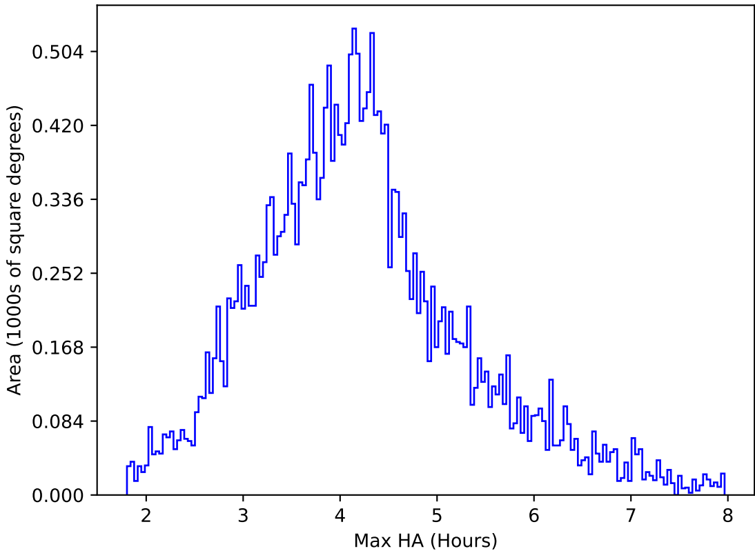
ddf_acor_sf30_lsf40_lsr10_v3.4_10yrs All sky r band: Max HA
