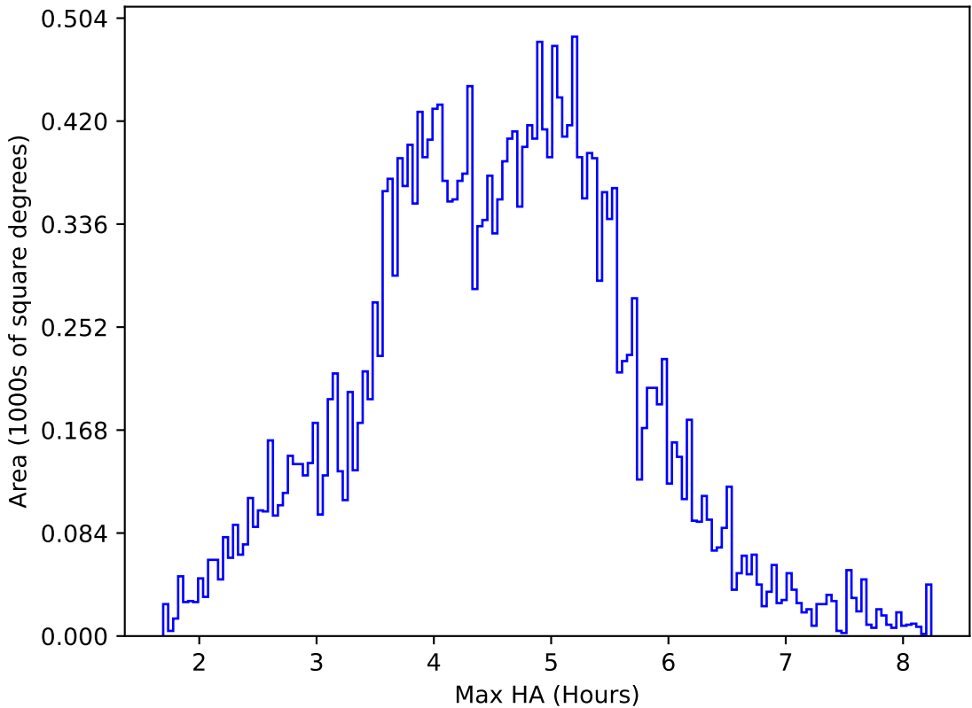
ddf_acor_sf30_lsf40_lsr10_v3.4_10yrs All sky i band: Max HA
