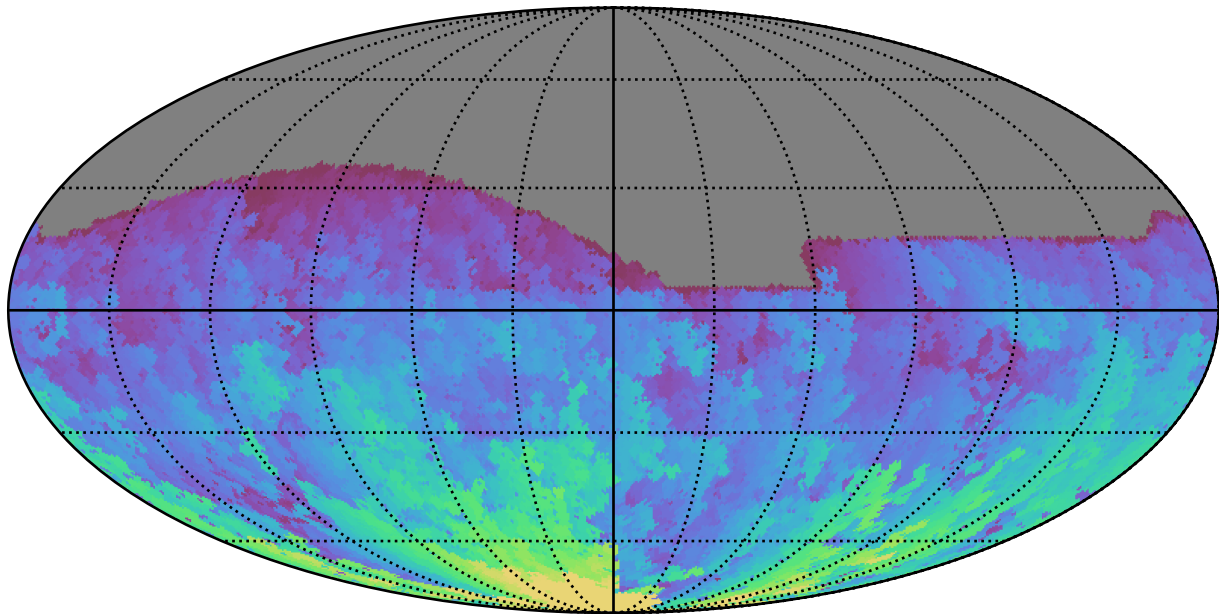
ddf_acor_sf30_lsf40_lsr10_v3.4_10yrs All sky g band: Max HA
