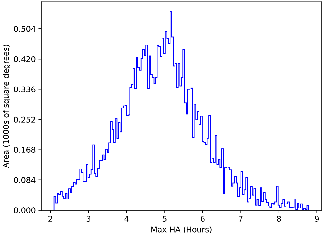
ddf_acor_sf30_lsf40_lsr10_v3.4_10yrs All sky all bands: Max HA
