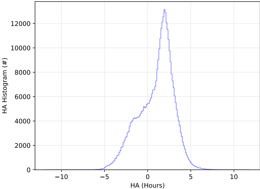
ddf_acor_sf30_lsf40_lsr10_v3.4_10yrs WFD y band: HA Histogram
