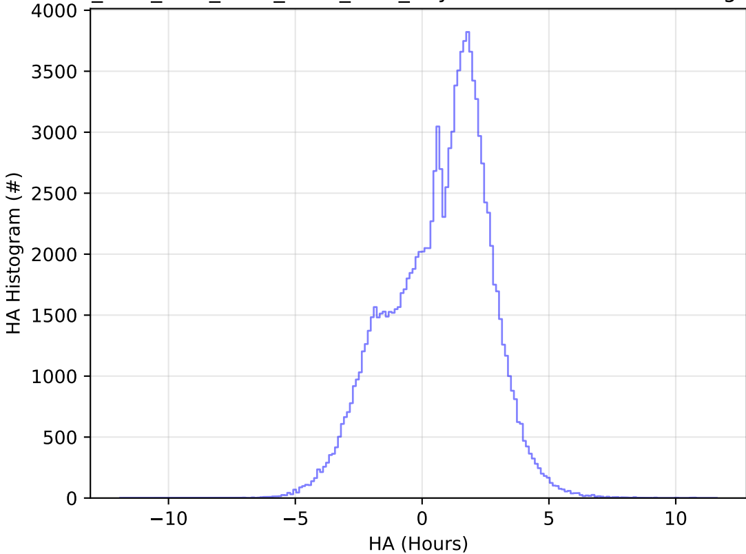
ddf_acor_sf30_lsf40_lsr10_v3.4_10yrs WFD u band: HA Histogram
