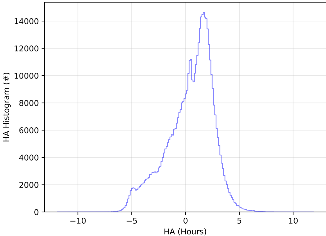
ddf_acor_sf30_lsf40_lsr10_v3.4_10yrs WFD r band: HA Histogram
