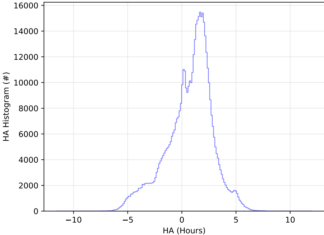
ddf_acor_sf30_ls40_lsr10_v3.4_10yrs WFD i band: HA Histogram
