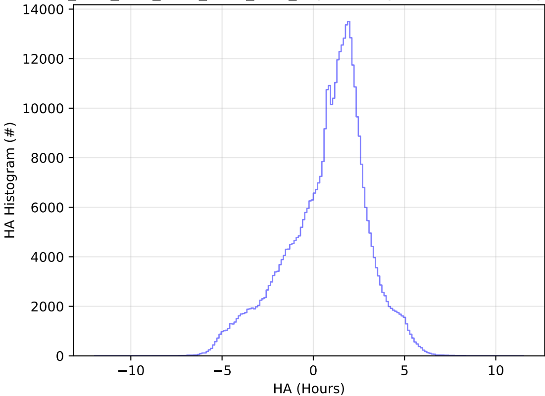
ddf_acor_sf30_lsf40_lsr10_v3.4_10yrs All sky z band: HA Histogram
