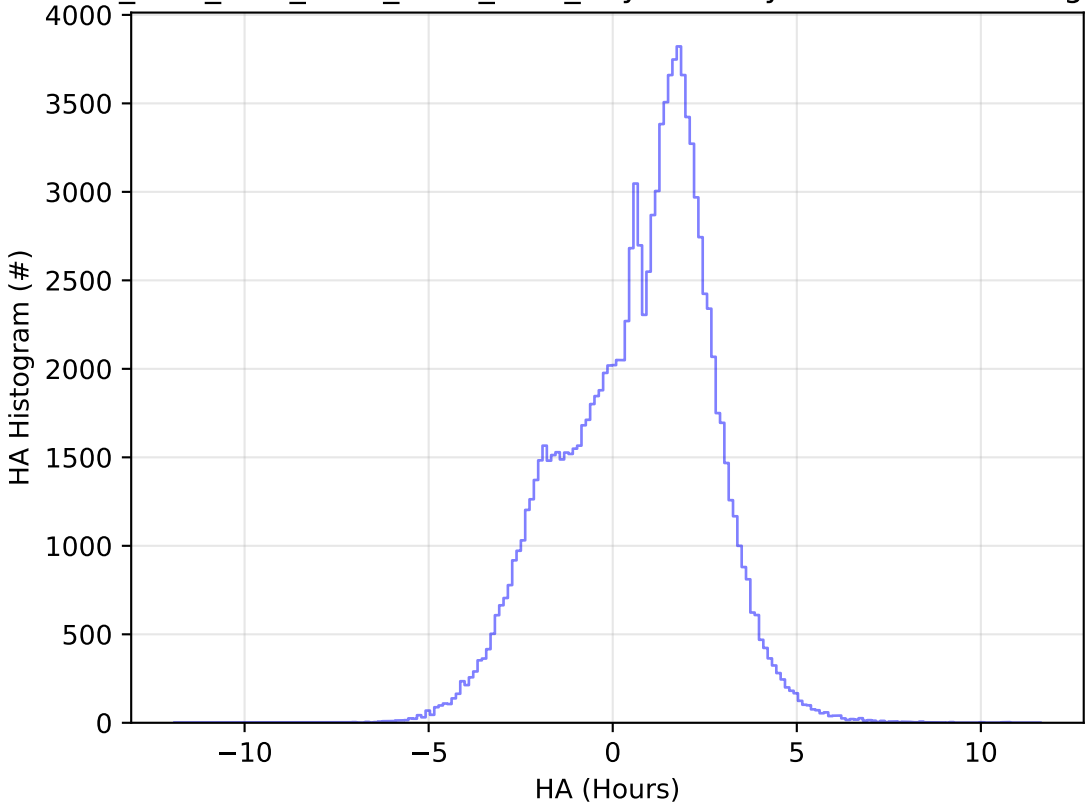
ddf_acor_sf30_lsf40_lsr10_v3.4_10yrs All sky u band: HA Histogram
