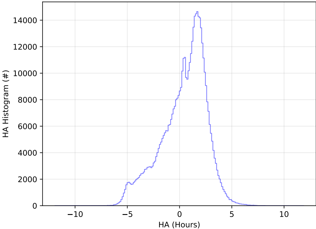
ddf_acor_sf30_lsf40_lsr10_v3.4_10yrs All sky r band: HA Histogram
