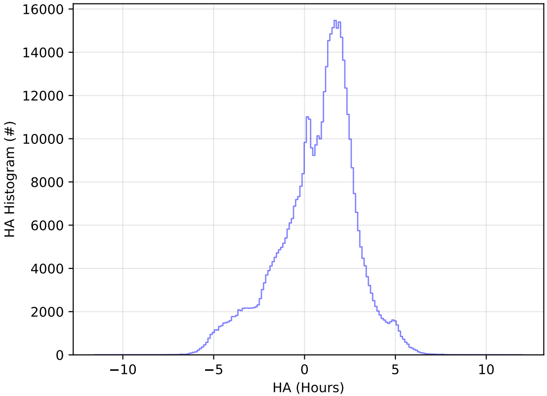
ddf_acor_sf30_lsf40_lsr10_v3.4_10yrs All sky i band: HA Histogram
