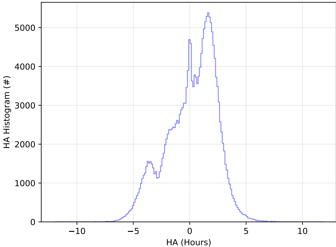
ddf_acor_sf30_lsf40_lsr10_v3.4_10yrs All sky g band: HA Histogram
