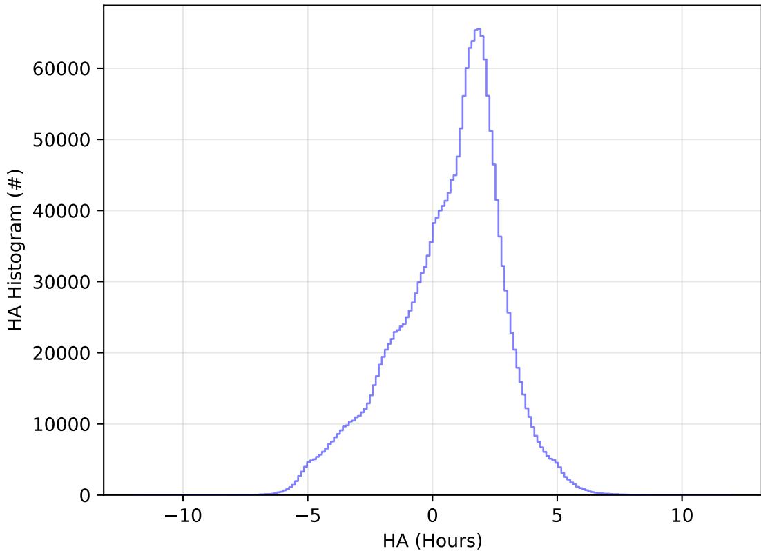
ddf_acor_sf30_lsf40_lsr10_v3.4_10yrs All sky all bands: HA Histogram
