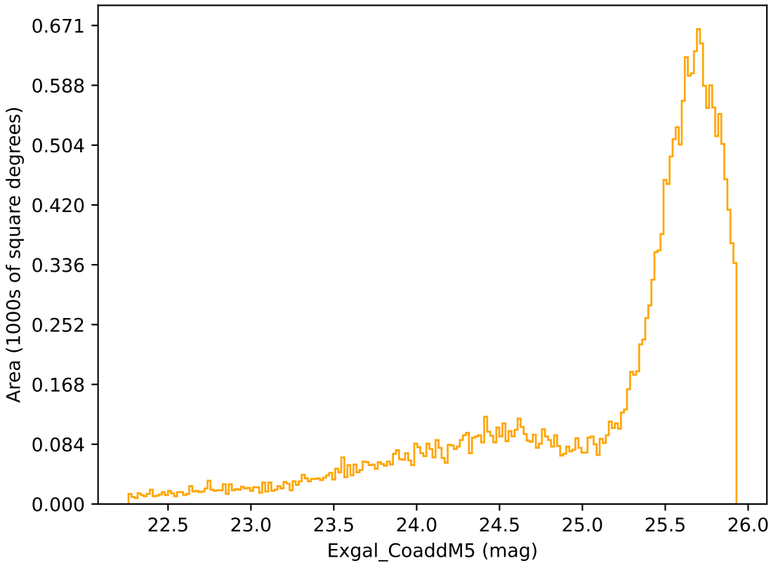
ddf_acor_sf30_lsf40_lsr10_v3.4_10yrs Yr 1 r band: Exgal_CoaddM5
