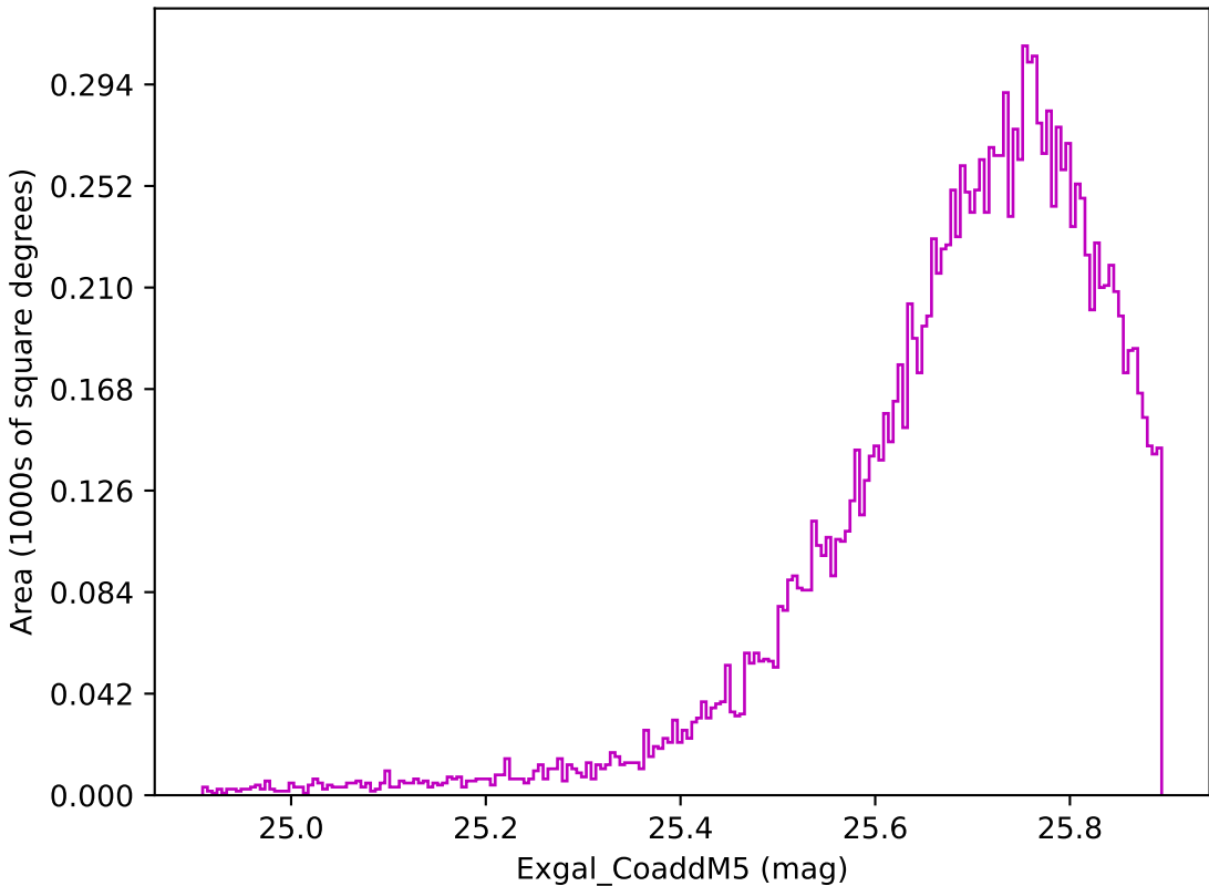
ddf_acor_sf30_lsf40_lsr10_v3.4_10yrs WFD z band: Exgal_CoaddM5
