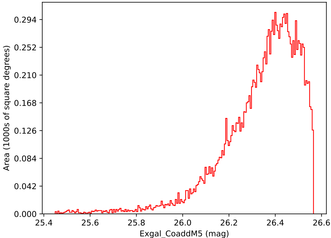
ddf_acor_sf30_lsf40_lsr10_v3.4_10yrs WFD i band: Exgal_CoaddM5
