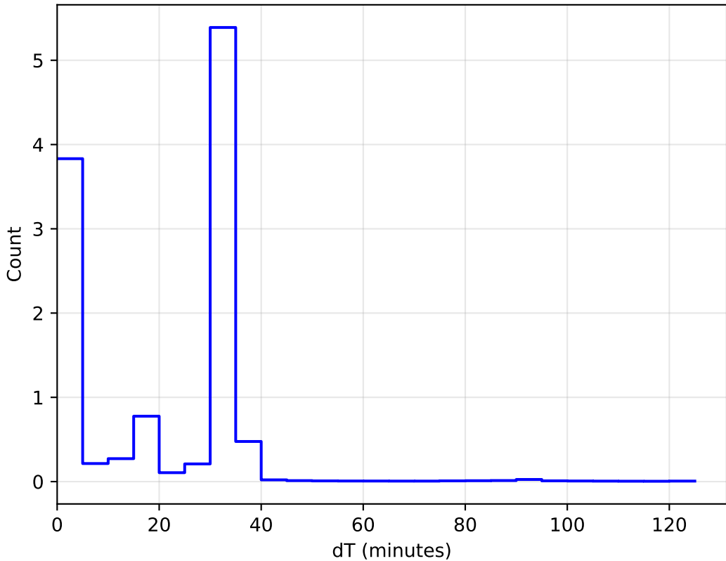
ddf_acor_sf30_lsf40_lsr10_v3.4_10yrs WFD: DeltaT Histogram 1e6
